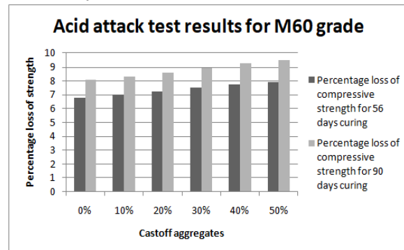
Acid attack test results
