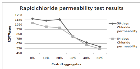
Rapid chloride permeability test results
