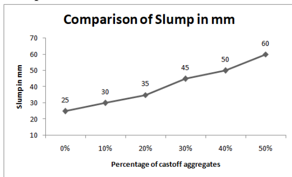
Comparison of slump cone test results
