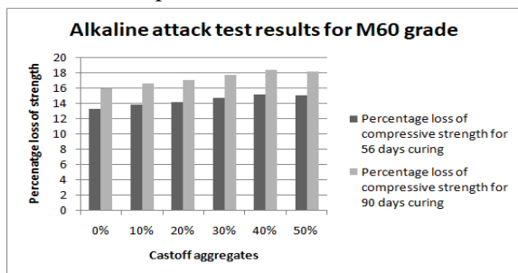
Alkaline attack test results
