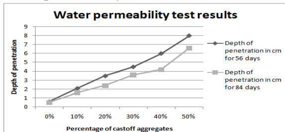
Water permeability test results
