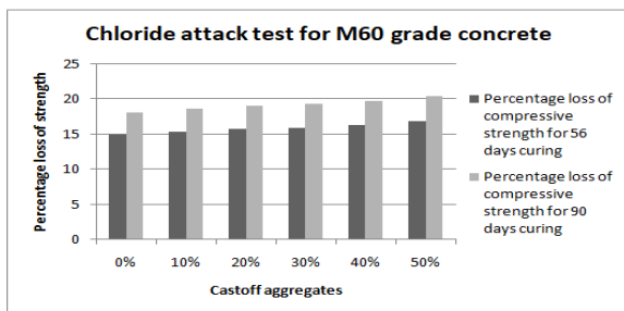
Chloride attack test results
