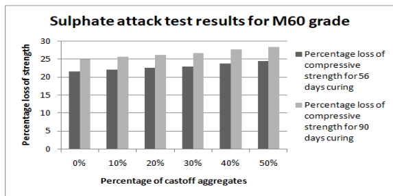
Sulphate attack test results
